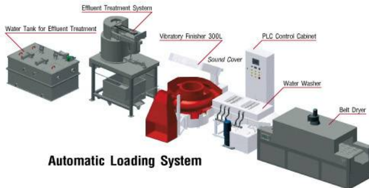
Vibratory Finishing Machine
